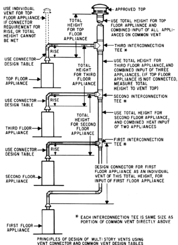
FIG. 23 - COMPLETE MULTI-STORY VENT SYSTEM
