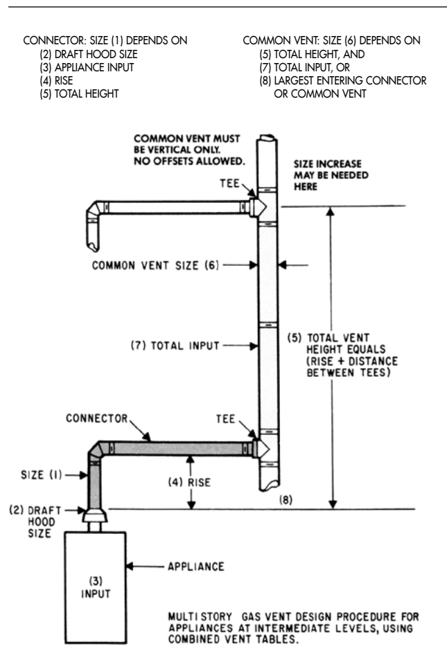
FIG. 22 - SYSTEM SEGMENT FOR MULTI-STORY VENT
